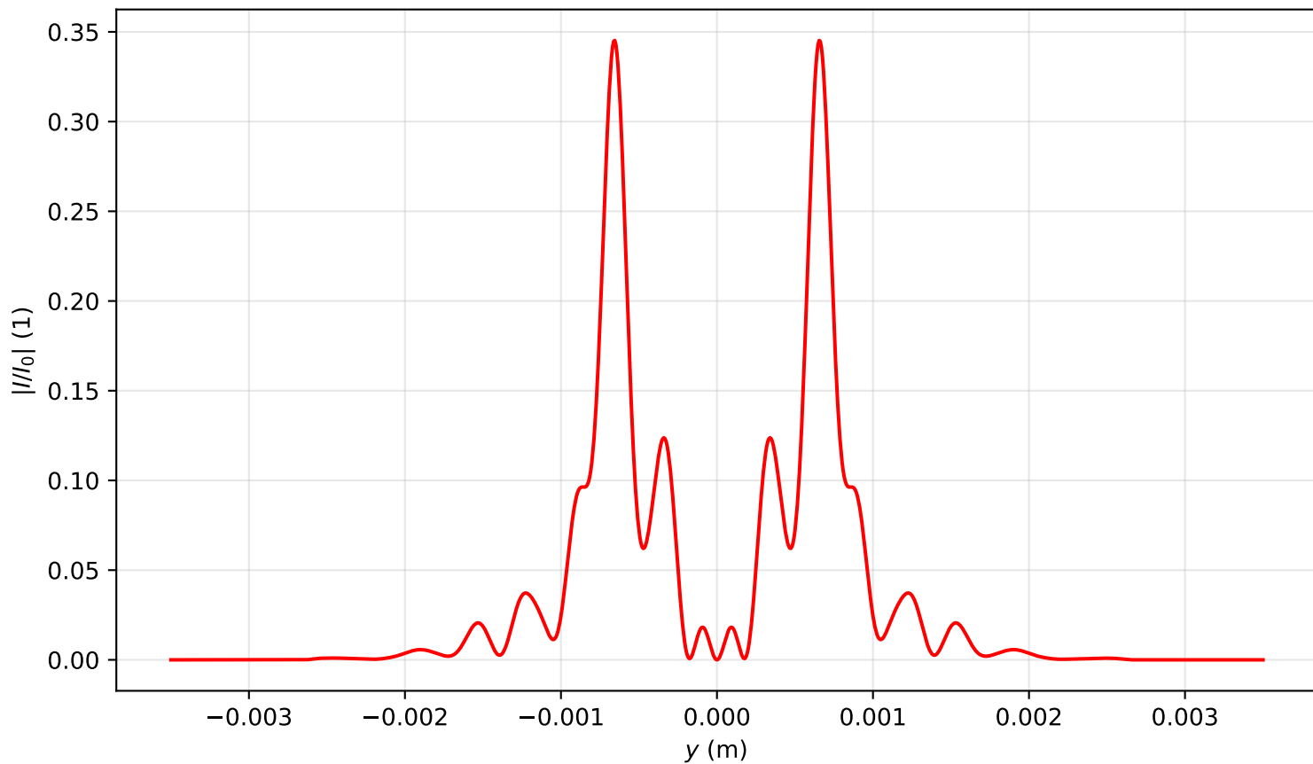
Intensity profile I(x=0, y, z=0.876)/I_0 , P_{in}=14.0\text{Pcr} , artificial time
