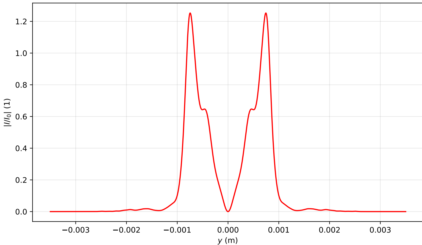
Intensity profile I(x=0, y, z=1.274)/I_0 , \text{Pin}=14.0\text{Pcr} , artificial time
