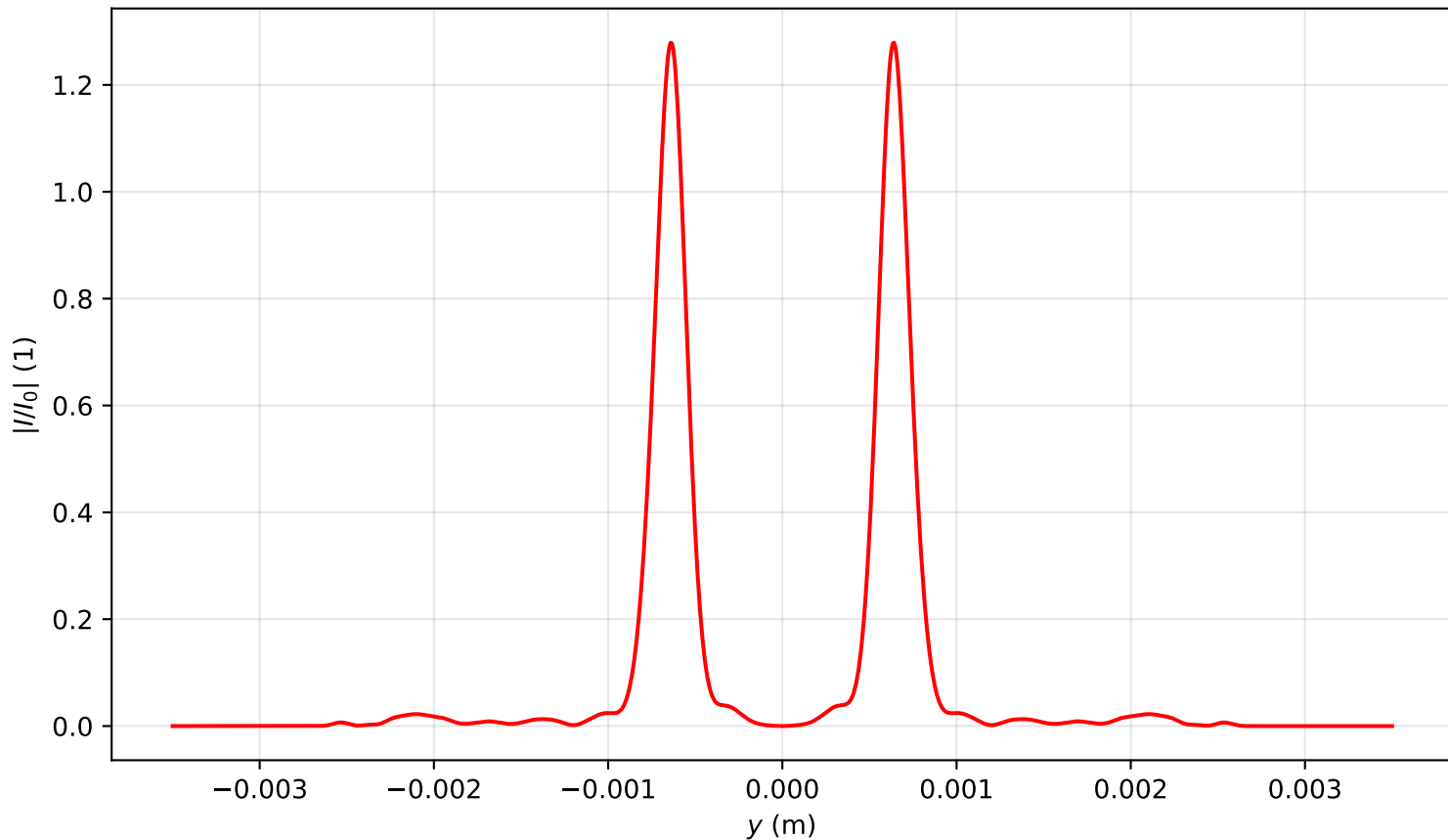
Intensity profile I(x=0, y, z=1.592)/I_0 , P_{in}=14.0P_{cr} , artificial time
