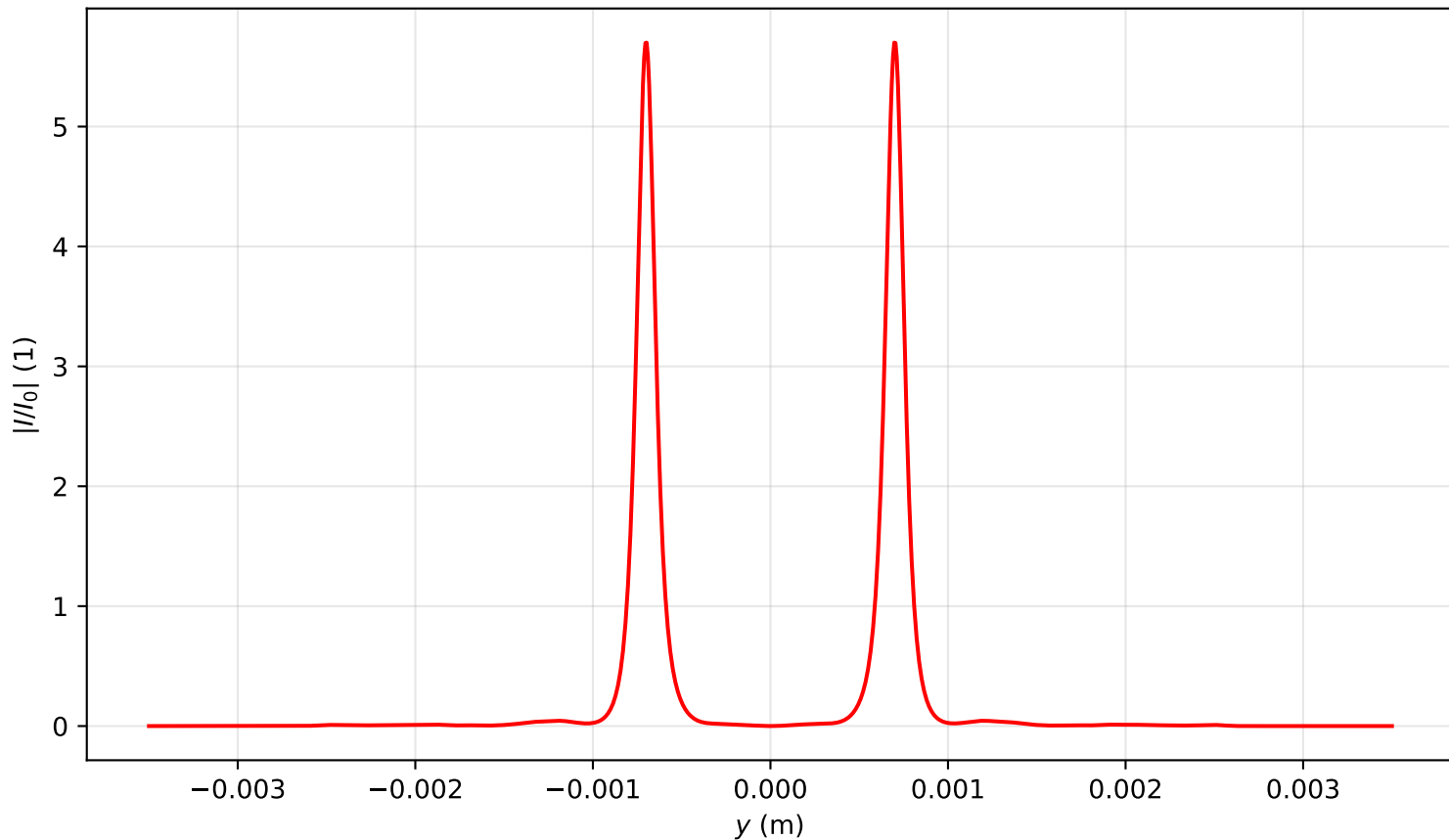
Intensity profile I(x=0, y, z=1.831)/I_0 , P_{in}=14.0P_{cr} , artificial time
