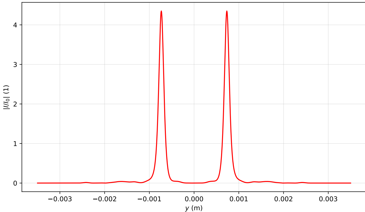
Intensity profile I(x=0, y, z=2.070)/I_0 , P_{in}=14.0P_{cr} , artificial time
