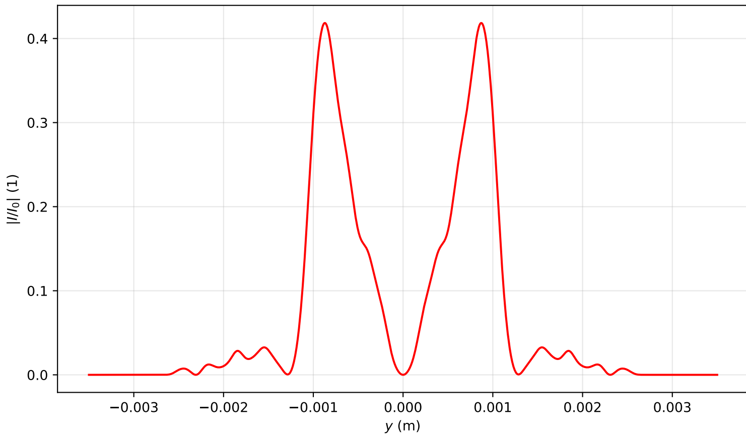
Intensity profile I(x=0, y, z=2.309)/I_0 , P_{in}=14.0P_{cr} , artificial time
