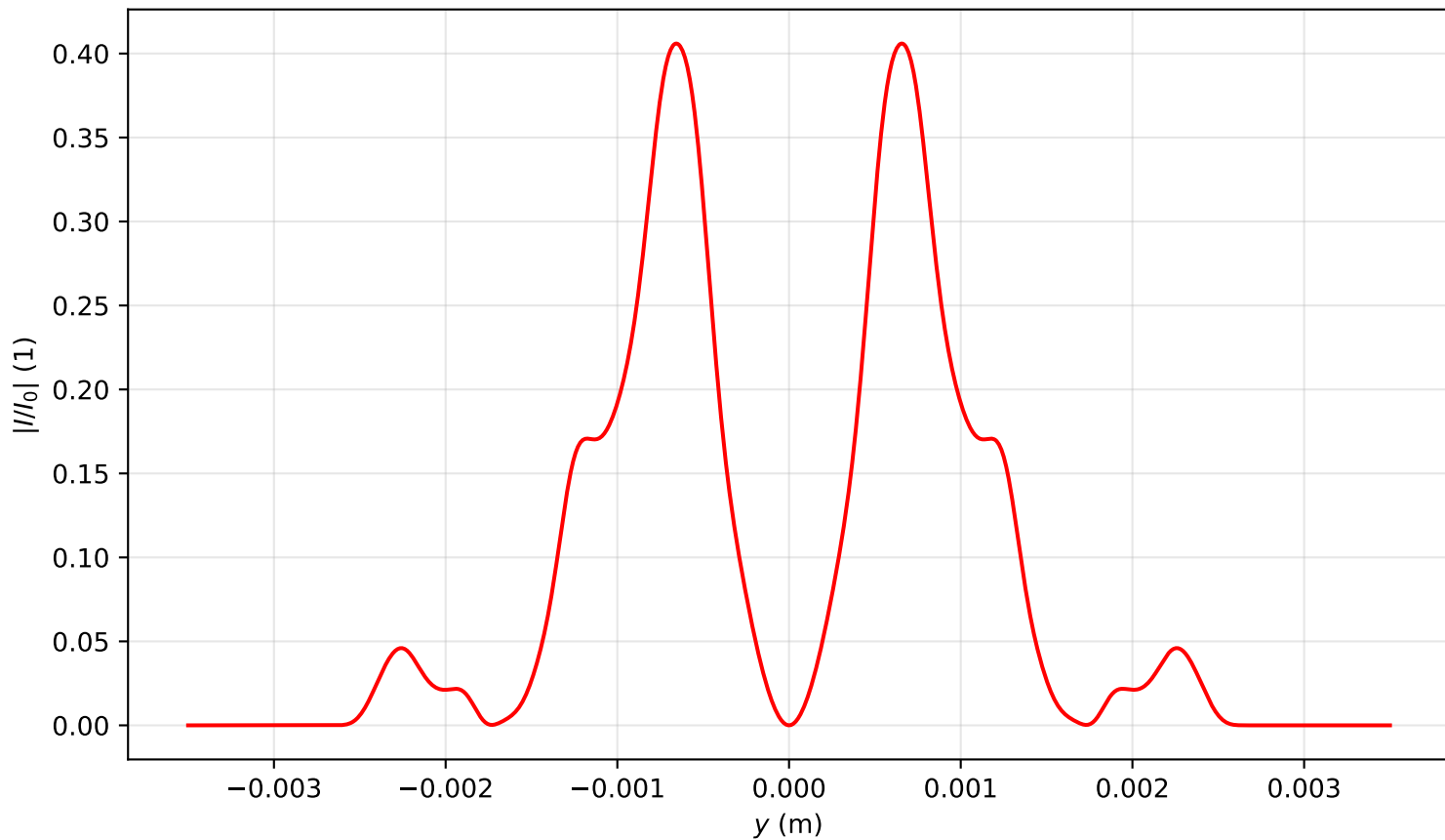
Intensity profile I(x = 0, y, z = 2.786)/I_0 , P_{in}=14.0\text{Pcr} , artificial time
