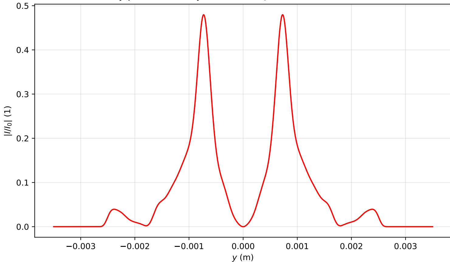
Intensity profile I(x=0, y, z=2.946)/I_0 , P_{in}=14.0P_{cr} , artificial time
