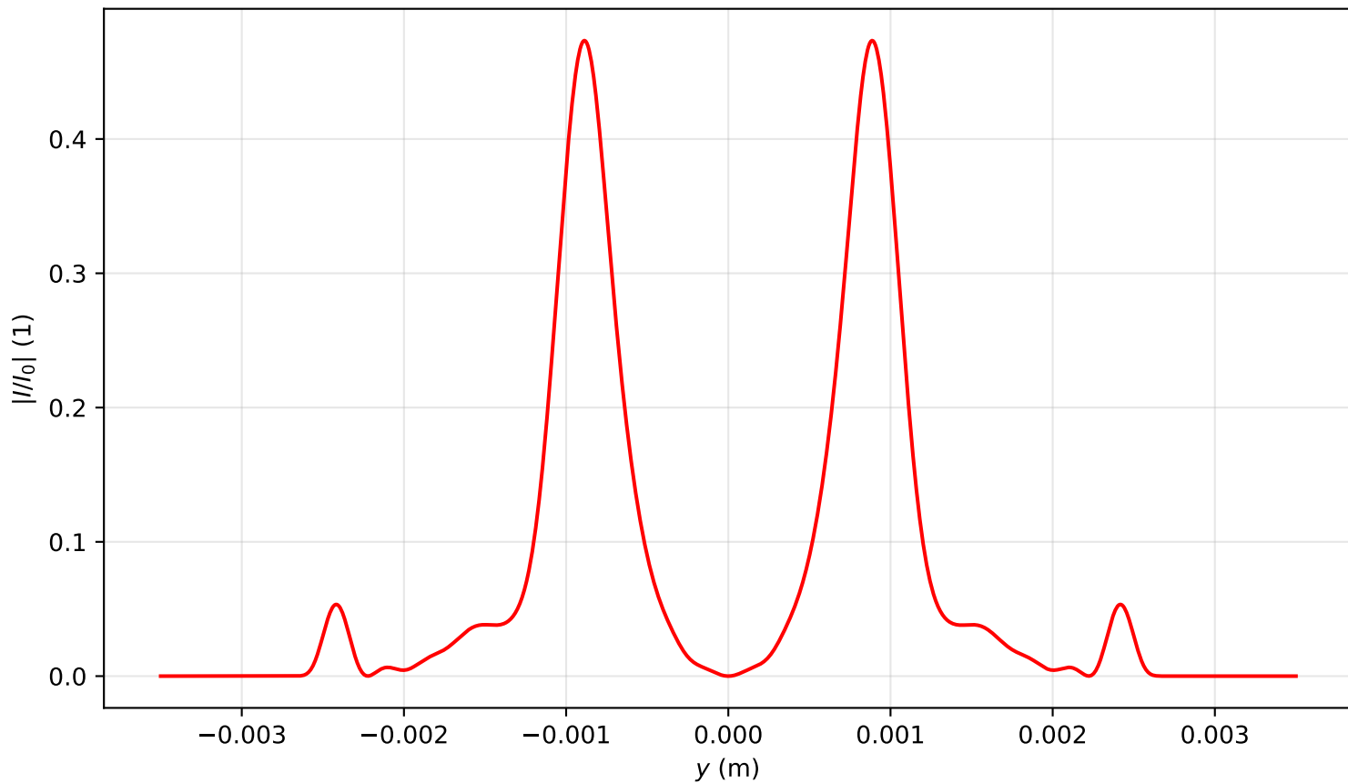
Intensity profile I(x=0, y, z=3.264)/I_0 , P_{in}=14.0\text{Pcr} , artificial time
