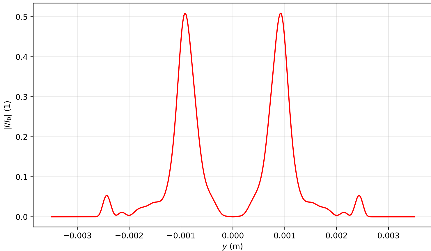
Intensity profile I(x=0, y, z=3.344)/I_0 , P_{in}=14.0\text{Pcr} , artificial time
