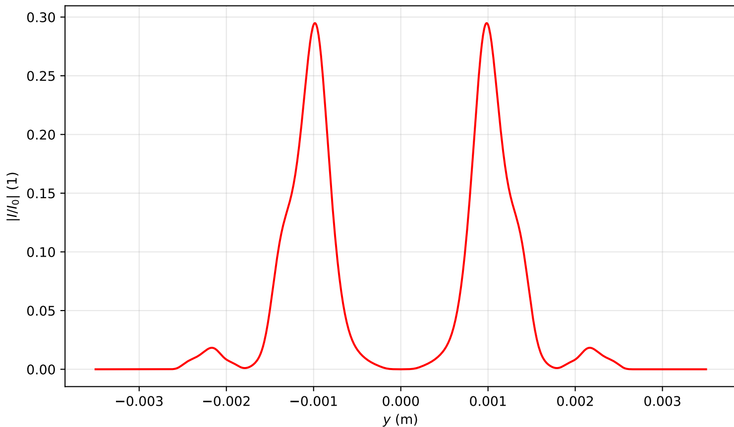
Intensity profile I(x=0, y, z=3.981)/I_0 , P_{in}=14.0\text{Pcr} , artificial time
