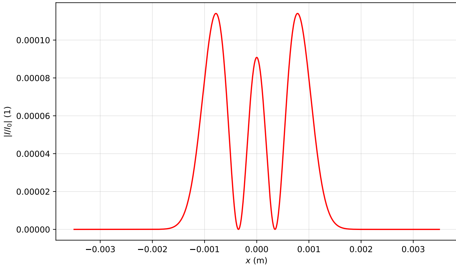
Intensity profile I(x, y = 0, z = 0.080)/I_0 , P_{in}=15.0P_{cr} , artificial time
