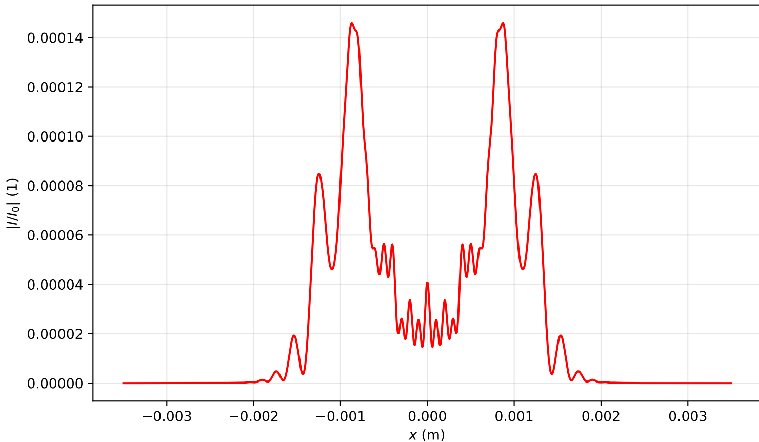
Intensity profile I(x, y = 0, z = 0.478)/I_0 , P_{in}=15.0P_{cr} , artificial time
