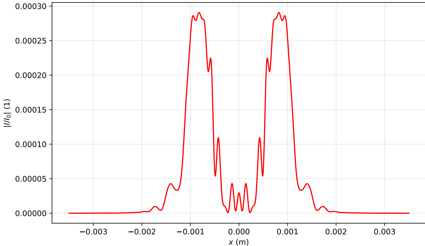
Intensity profile I(x, y = 0, z = 0.557)/I_0 , P_{in}=15.0P_{cr} , artificial time
