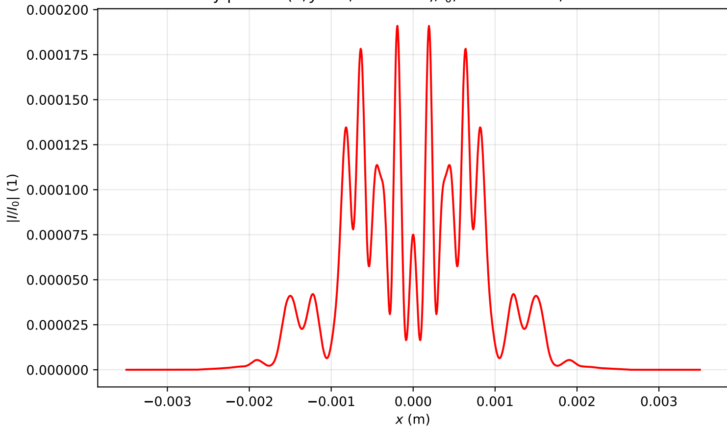
Intensity profile I(x, y = 0, z = 0.637)/I_0 , P_{in}=15.0P_{cr} , artificial time
