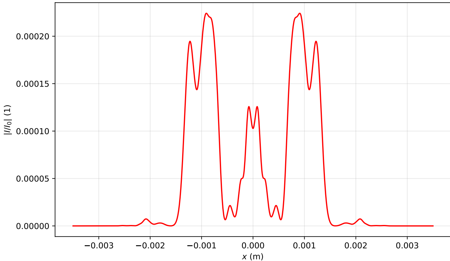
Intensity profile I(x, y = 0, z = 1.115)/I_0 , P_{in}=15.0P_{cr} , artificial time
