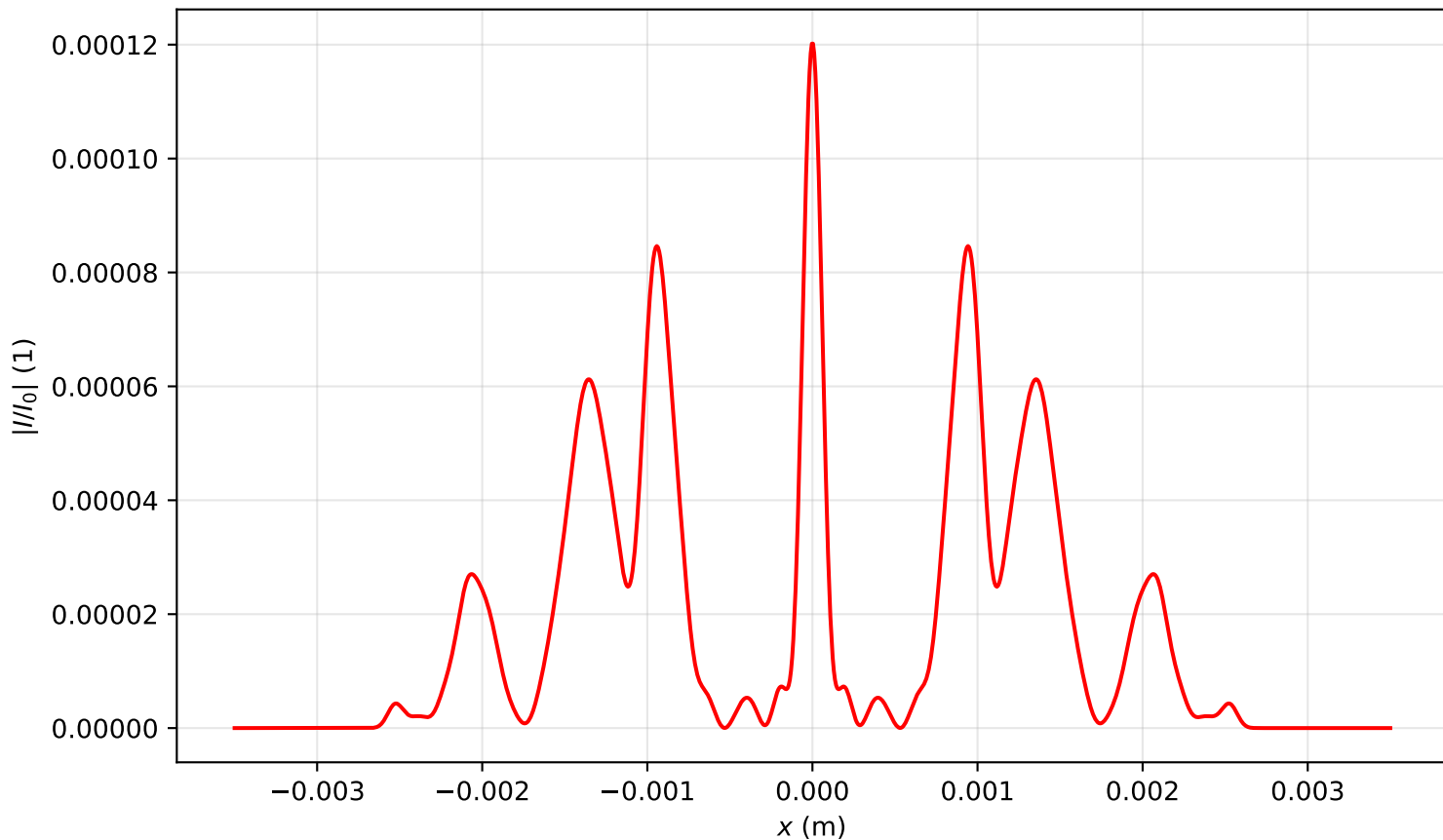
Intensity profile I(x, y = 0, z = 1.353)/I_0 , P_{in}=15.0P_{cr} , artificial time
