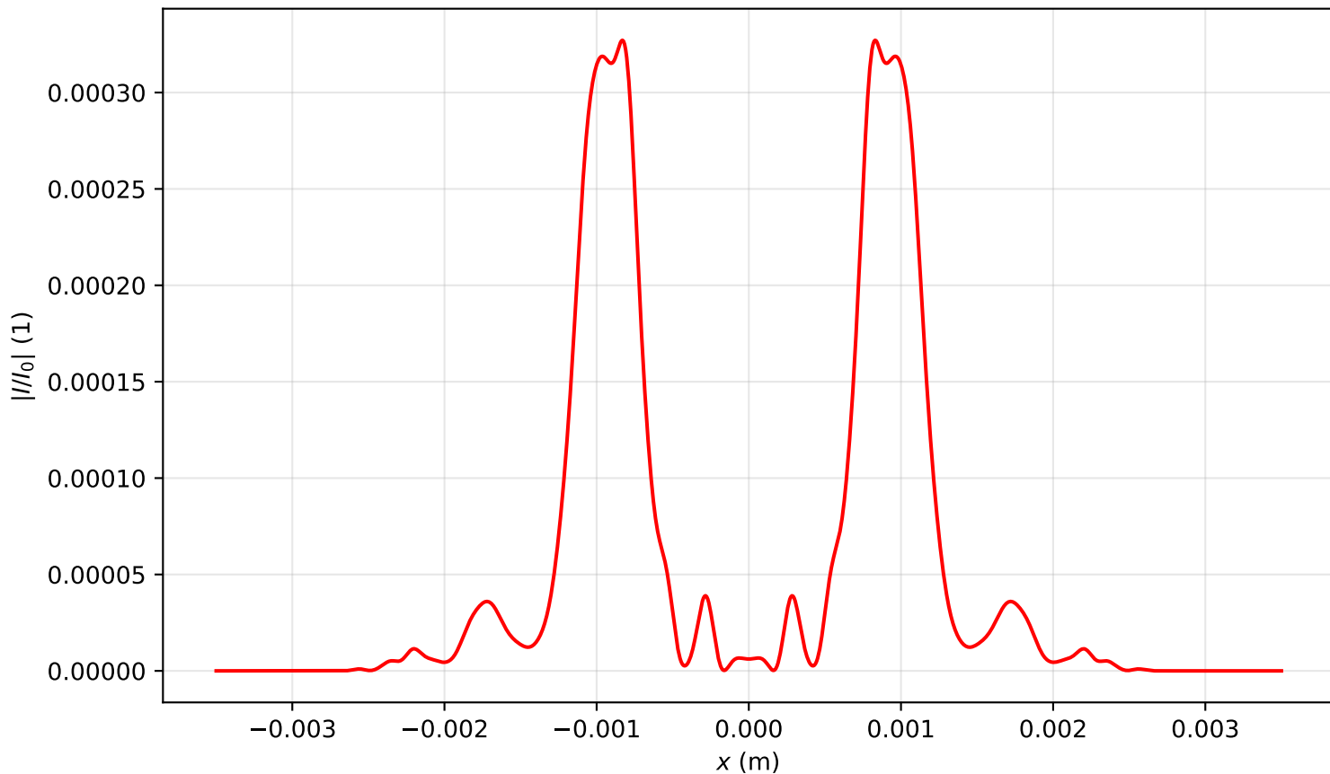
Intensity profile I(x, y = 0, z = 1.672)/I_0 , P_{in}=15.0P_{cr} , artificial time
