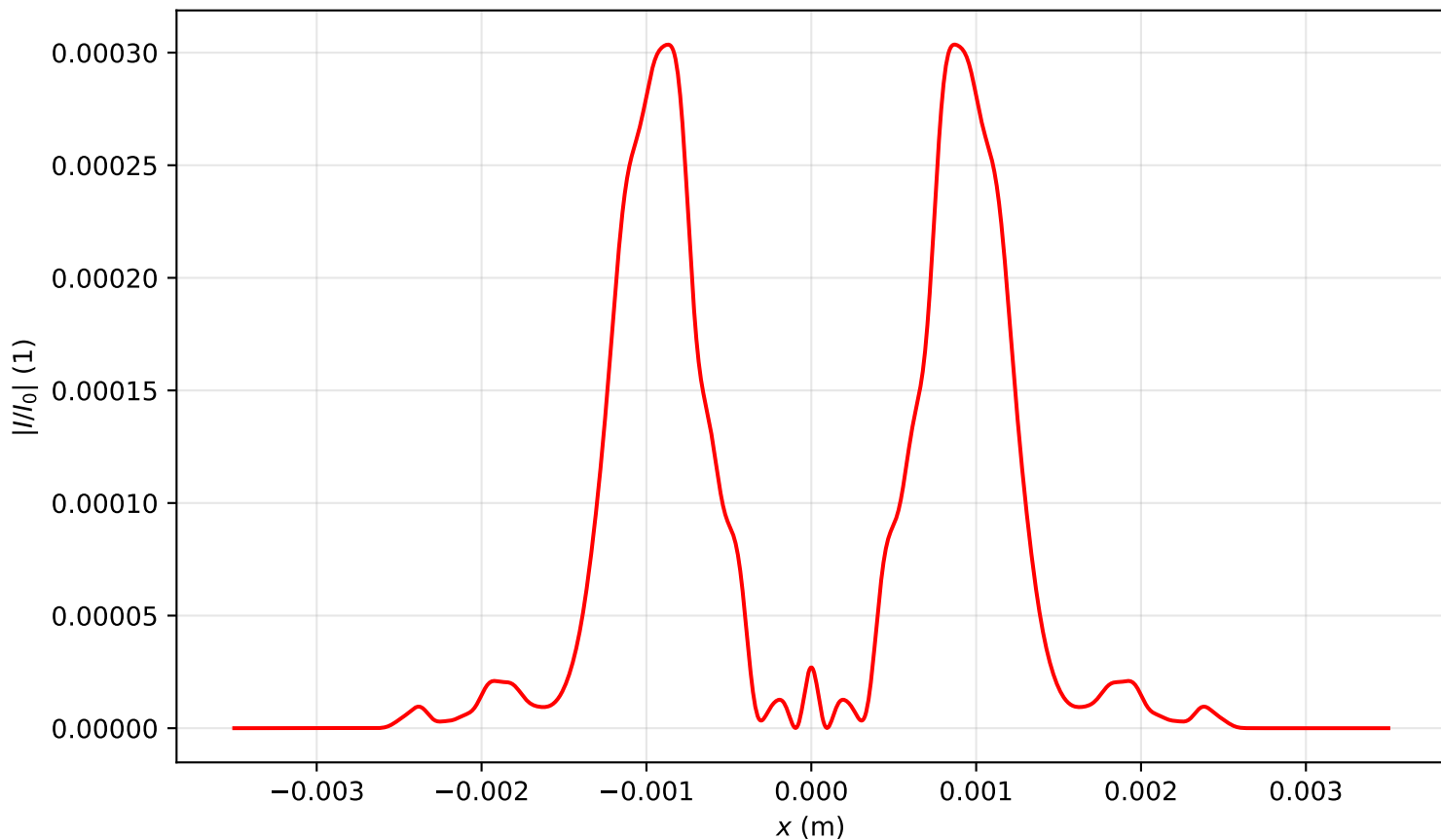
Intensity profile I(x, y = 0, z = 1.751)/I_0 , P_{in}=15.0P_{cr} , artificial time
