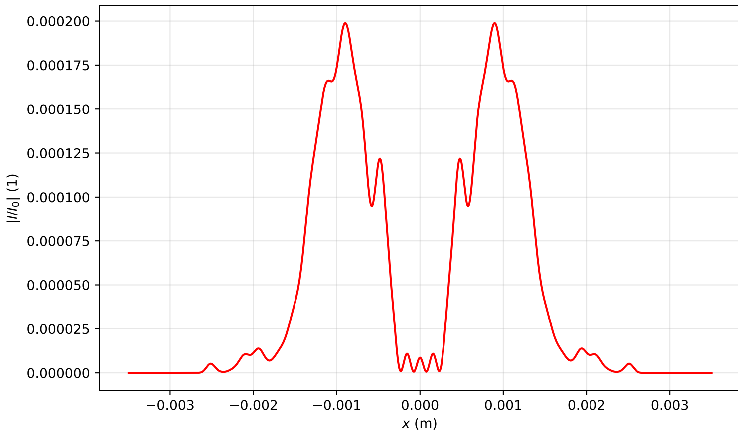
Intensity profile I(x, y = 0, z = 1.831)/I_0 , P_{in}=15.0\text{Pcr} , artificial time
