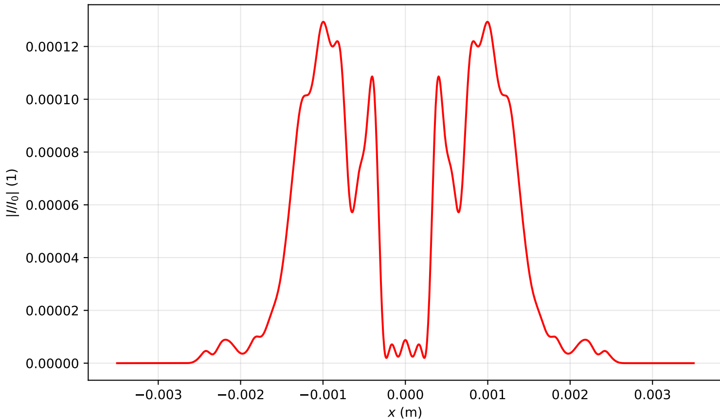
Intensity profile I(x, y = 0, z = 1.911)/I_0 , P_{in}=15.0\text{Pcr} , artificial time
