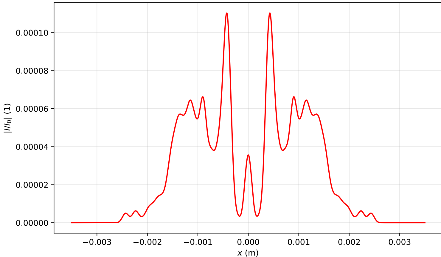
Intensity profile I(x, y = 0, z = 1.990)/I_0 , P_{in}=15.0P_{cr} , artificial time
