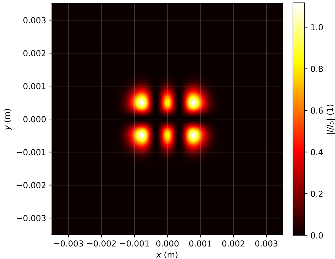
Intensity profile I(x, y, z = 0.080)/I_0 , P_{in}=15.0\text{Pcr} , artificial time
