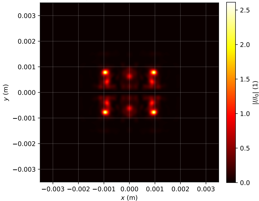
Intensity profile I(x, y, z = 1.035)/I_0 , P_{in}=15.0\text{Pcr} , artificial time
