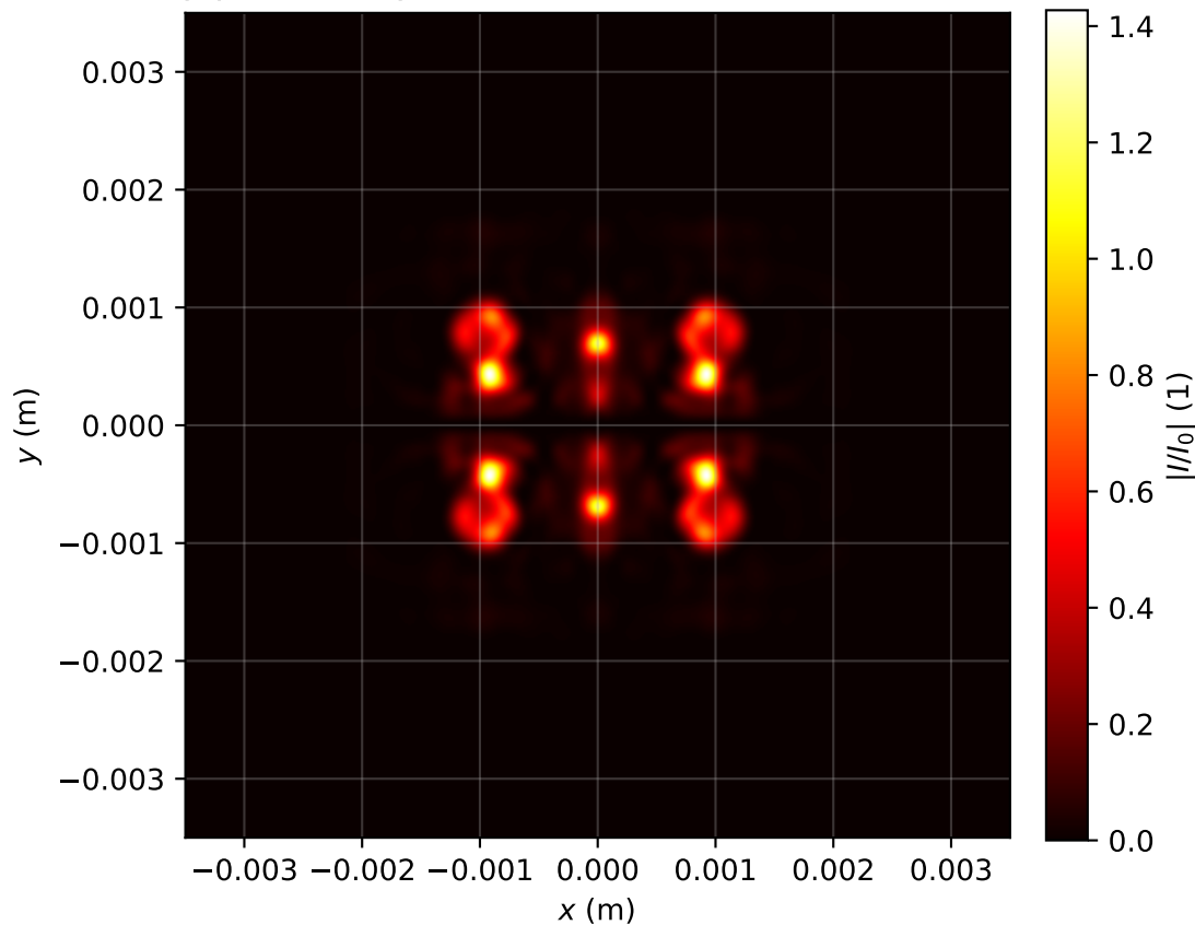
Intensity profile I(x, y, z = 1.115)/I_0 , P_{in}=15.0\text{Pcr} , artificial time
