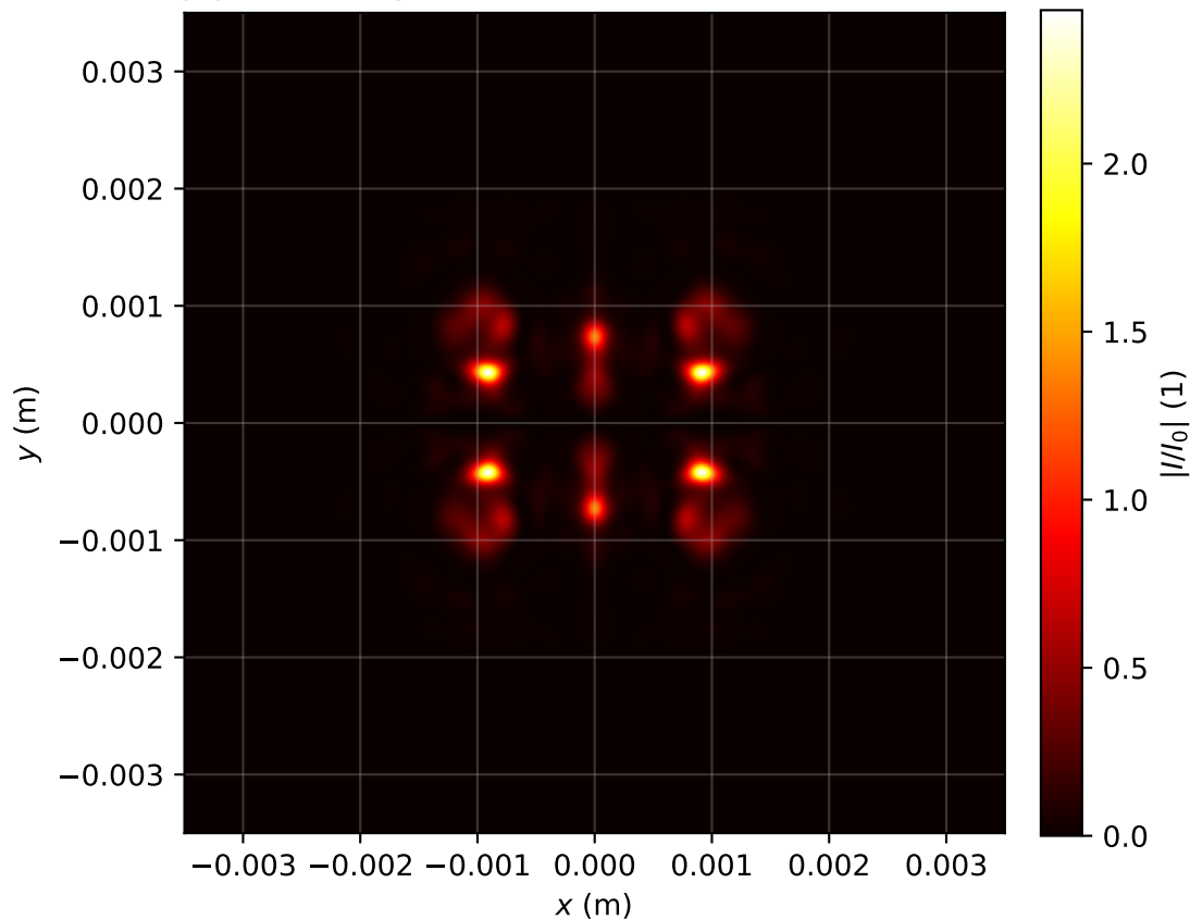
Intensity profile I(x, y, z = 1.194)/I_0 , P_{in}=15.0\text{Pcr} , artificial time
