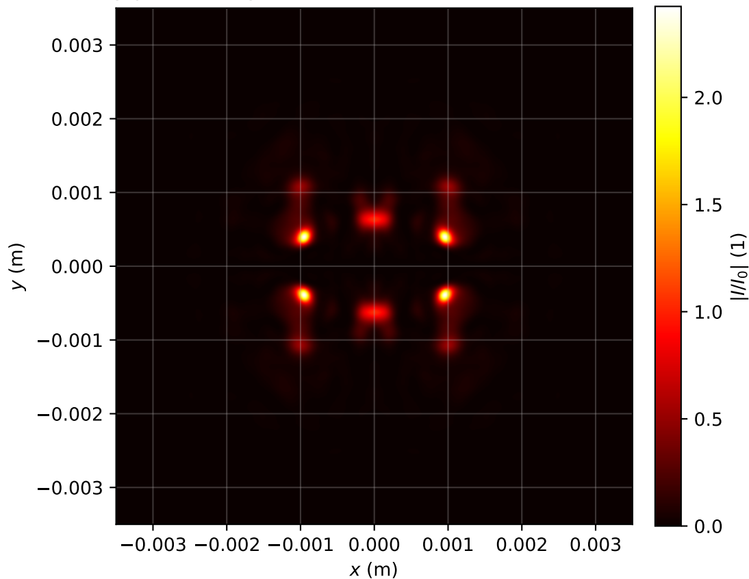
Intensity profile I(x, y, z = 1.513)/I_0 , P_{in}=15.0\text{Pcr} , artificial time
