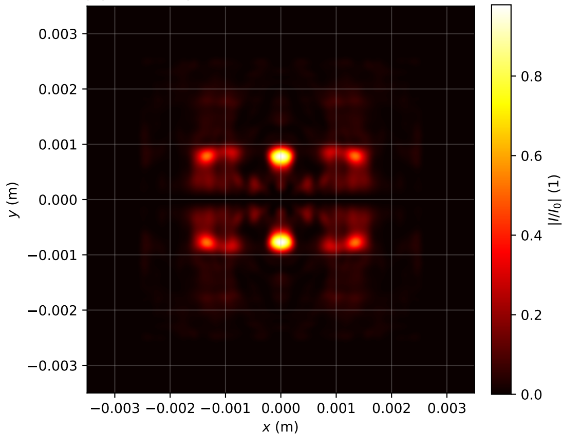
Intensity profile I(x, y, z = 2.070)/I_0 , P_{in}=15.0\text{Pcr} , artificial time
