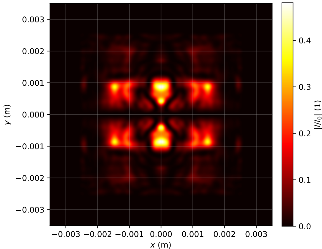
Intensity profile I(x, y, z = 2.229)/I_0 , P_{in}=15.0P_{cr} , artificial time
