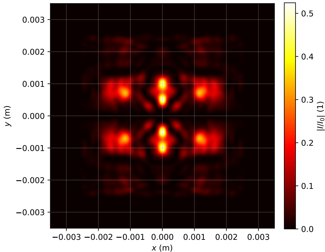
Intensity profile I(x, y, z = 2.388)/I_0 , P_{in}=15.0\text{Pcr} , artificial time
