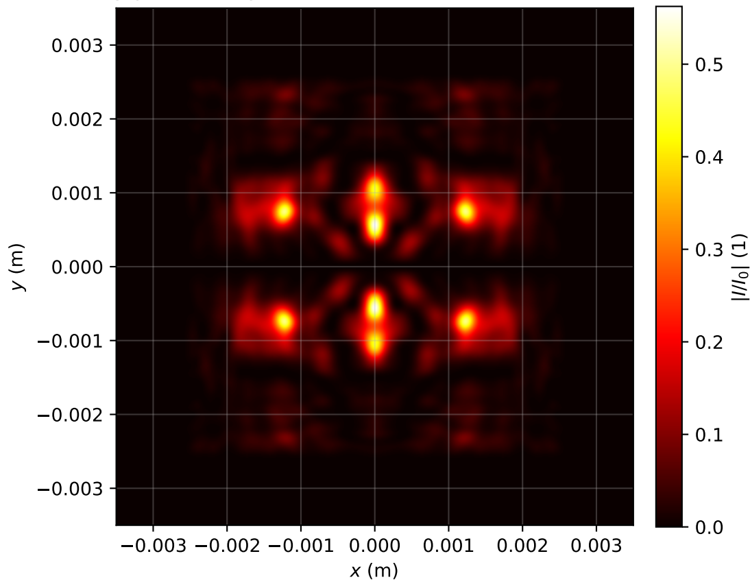
Intensity profile I(x, y, z = 2.468)/I_0 , P_{in}=15.0\text{Pcr} , artificial time
