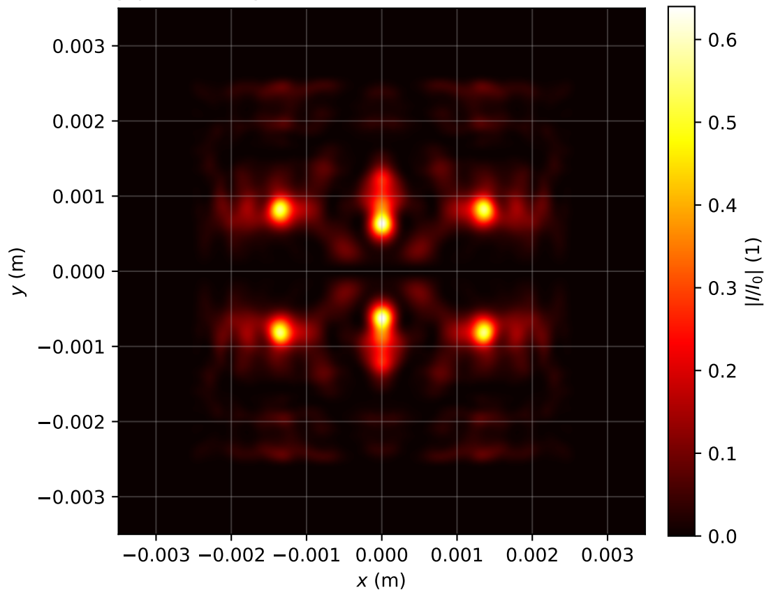
Intensity profile I(x, y, z = 2.627)/I_0 , P_{in}=15.0P_{cr} , artificial time
