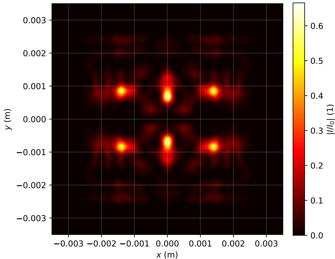
Intensity profile I(x, y, z = 2.707)/I_0 , P_{in}=15.0P_{cr} , artificial time
