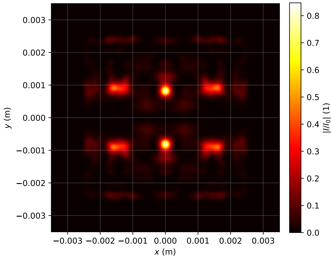
Intensity profile I(x, y, z = 2.946)/I_0 , P_{in}=15.0\text{Pcr} , artificial time
