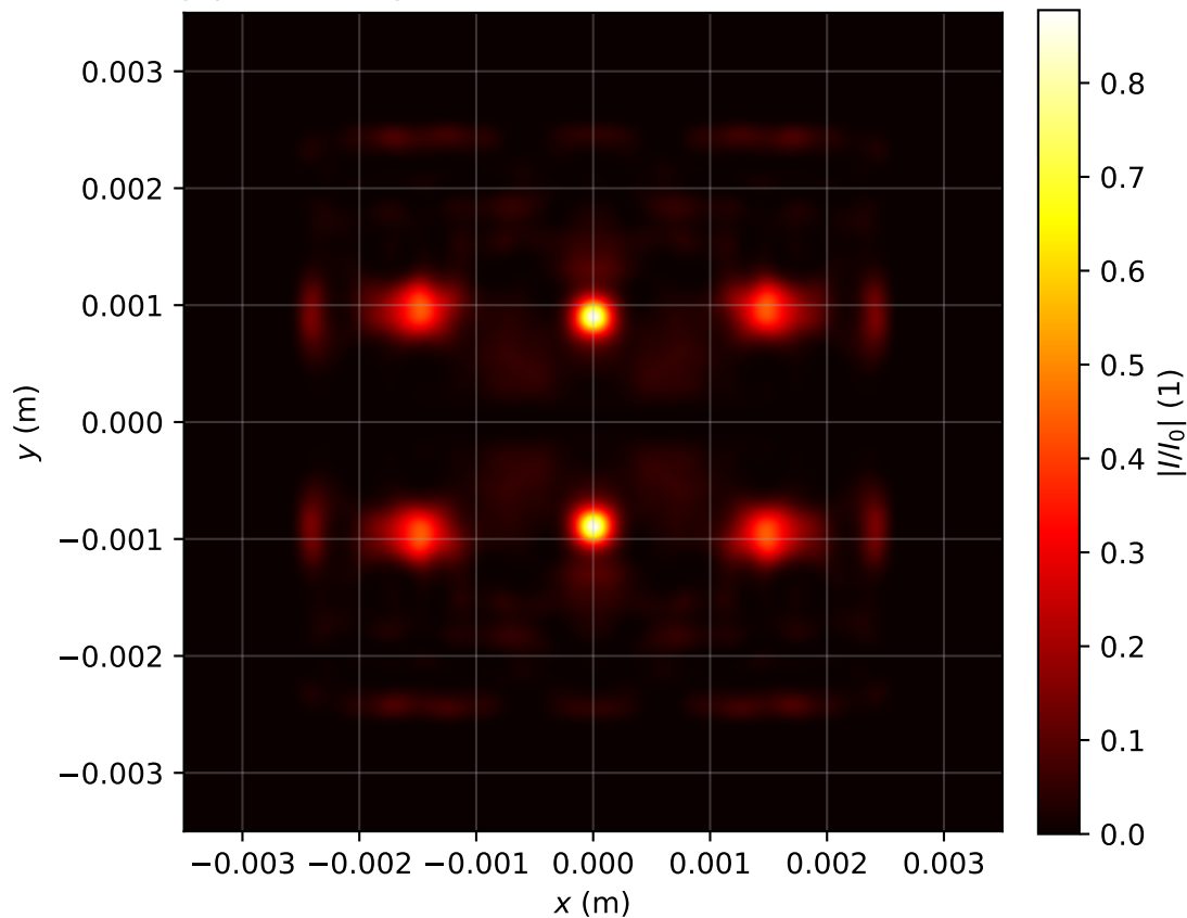
Intensity profile I(x, y, z = 3.105)/I_0 , P_{in}=15.0\text{Pcr} , artificial time
