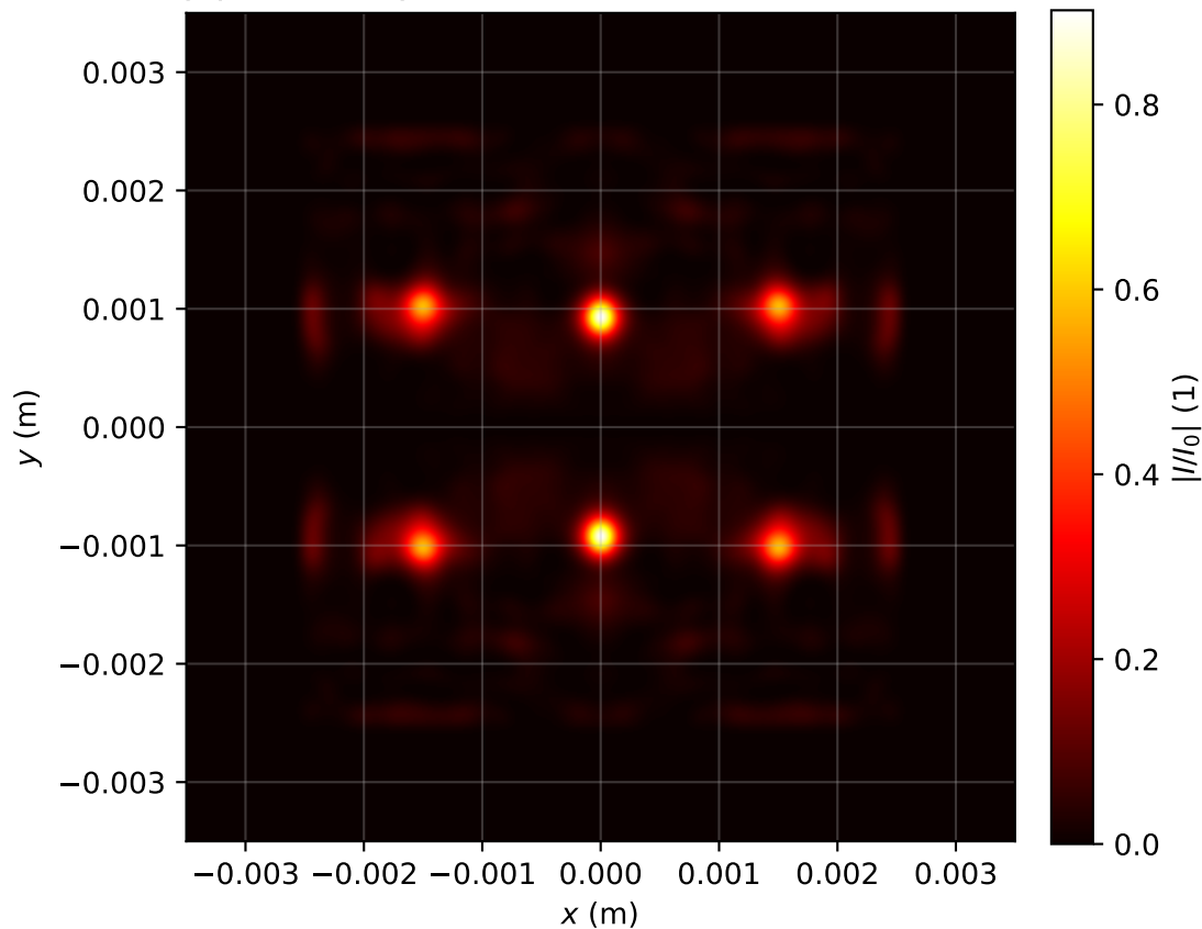
Intensity profile I(x, y, z = 3.184)/I_0 , P_{in}=15.0\text{Pcr} , artificial time
