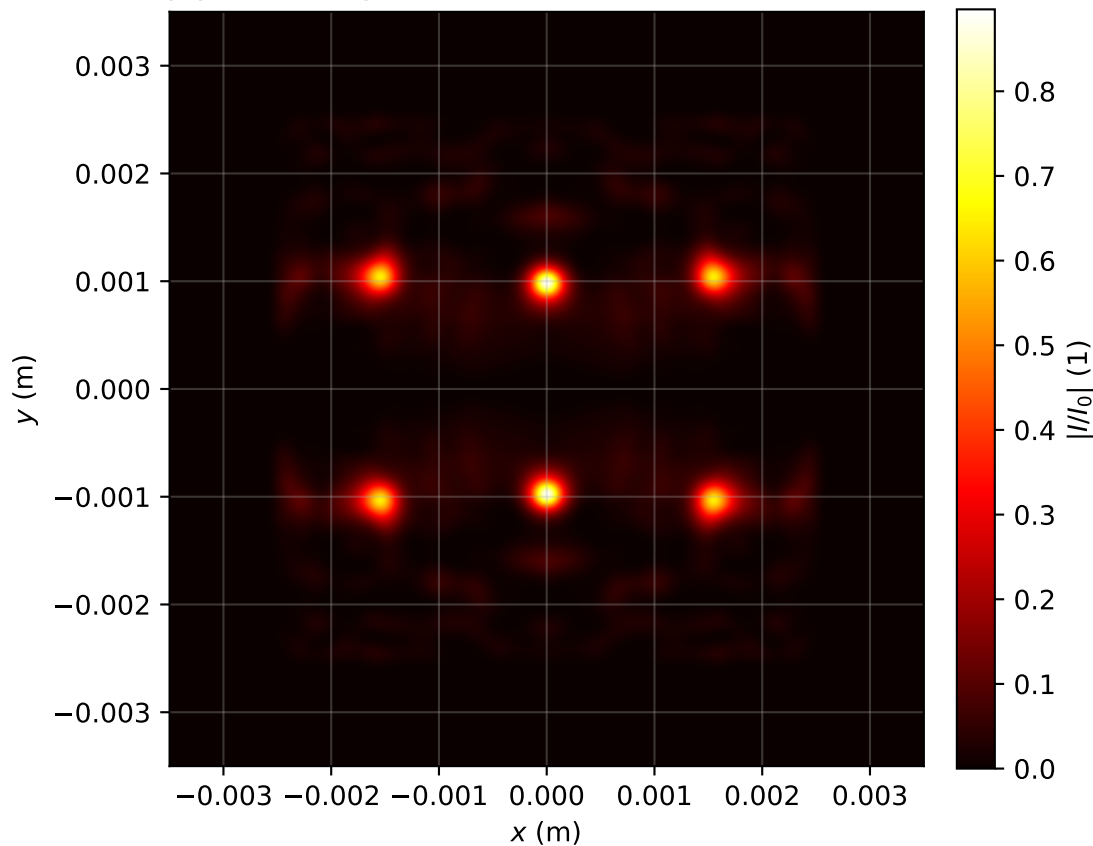
Intensity profile I(x, y, z = 3.344)/I_0 , P_{in}=15.0\text{Pcr} , artificial time
