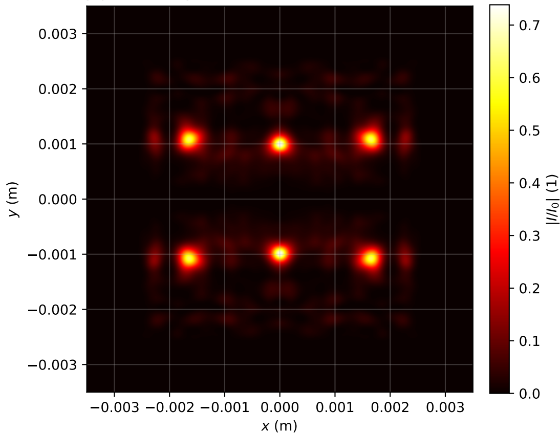
Intensity profile I(x, y, z = 3.503)/I_0 , P_{in}=15.0P_{cr} , artificial time
