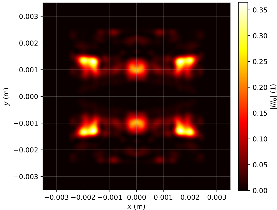
Intensity profile I(x, y, z = 3.981)/I_0 , P_{in}=15.0\text{Pcr} , artificial time
