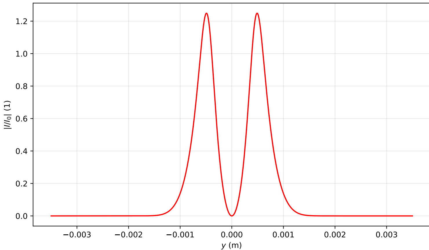
Intensity profile I(x=0, y, z=0.159)/I_0 , P_{in}=15.0P_{cr} , artificial time
