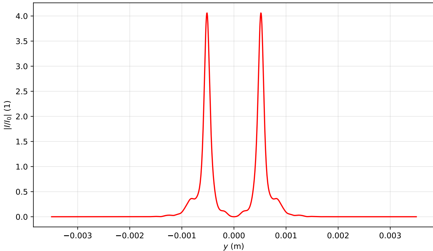
Intensity profile I(x=0, y, z=0.557)/I_0 , P_{in}=15.0P_{cr} , artificial time
