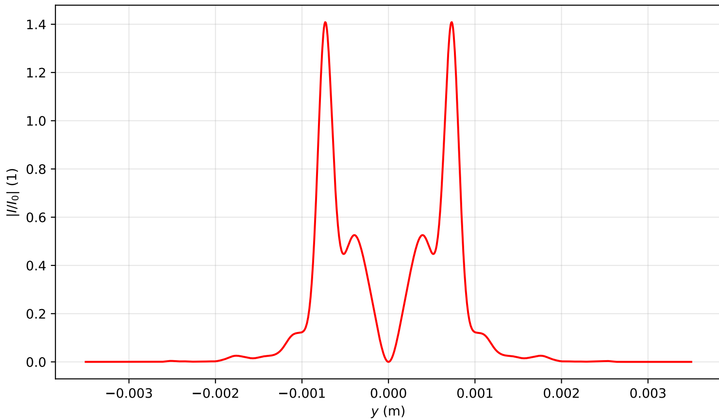
Intensity profile I(x=0, y, z=1.194)/I_0 , P_{in}=15.0P_{cr} , artificial time
