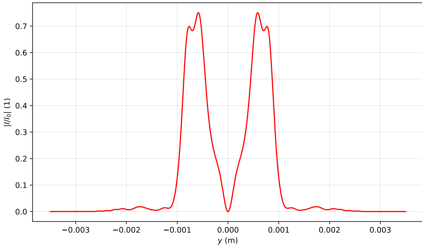
Intensity profile I(x=0, y, z=1.353)/I_0 , P_{in}=15.0P_{cr} , artificial time
