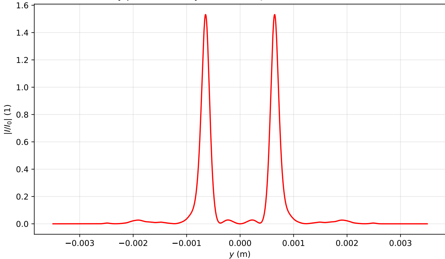
Intensity profile I(x=0, y, z=1.592)/I_0 , P_{in}=15.0P_{cr} , artificial time
