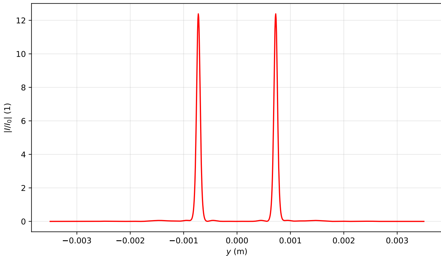
Intensity profile I(x = 0, y, z = 1.911)/I_0 , P_{in}=15.0\text{Pcr} , artificial time
