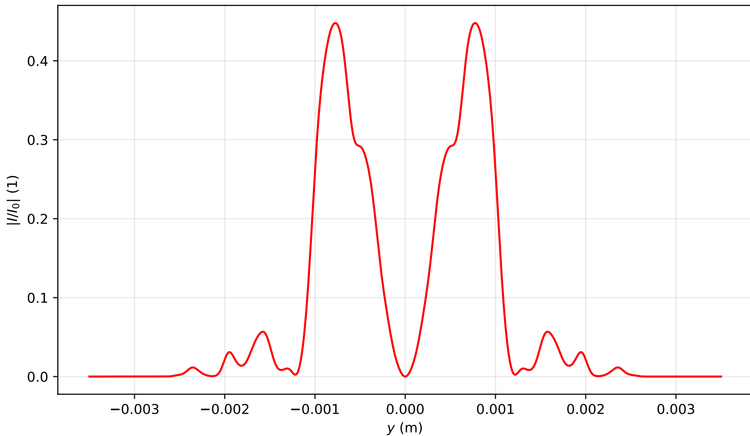
Intensity profile I(x=0, y, z=2.149)/I_0 , P_{in}=15.0P_{cr} , artificial time
