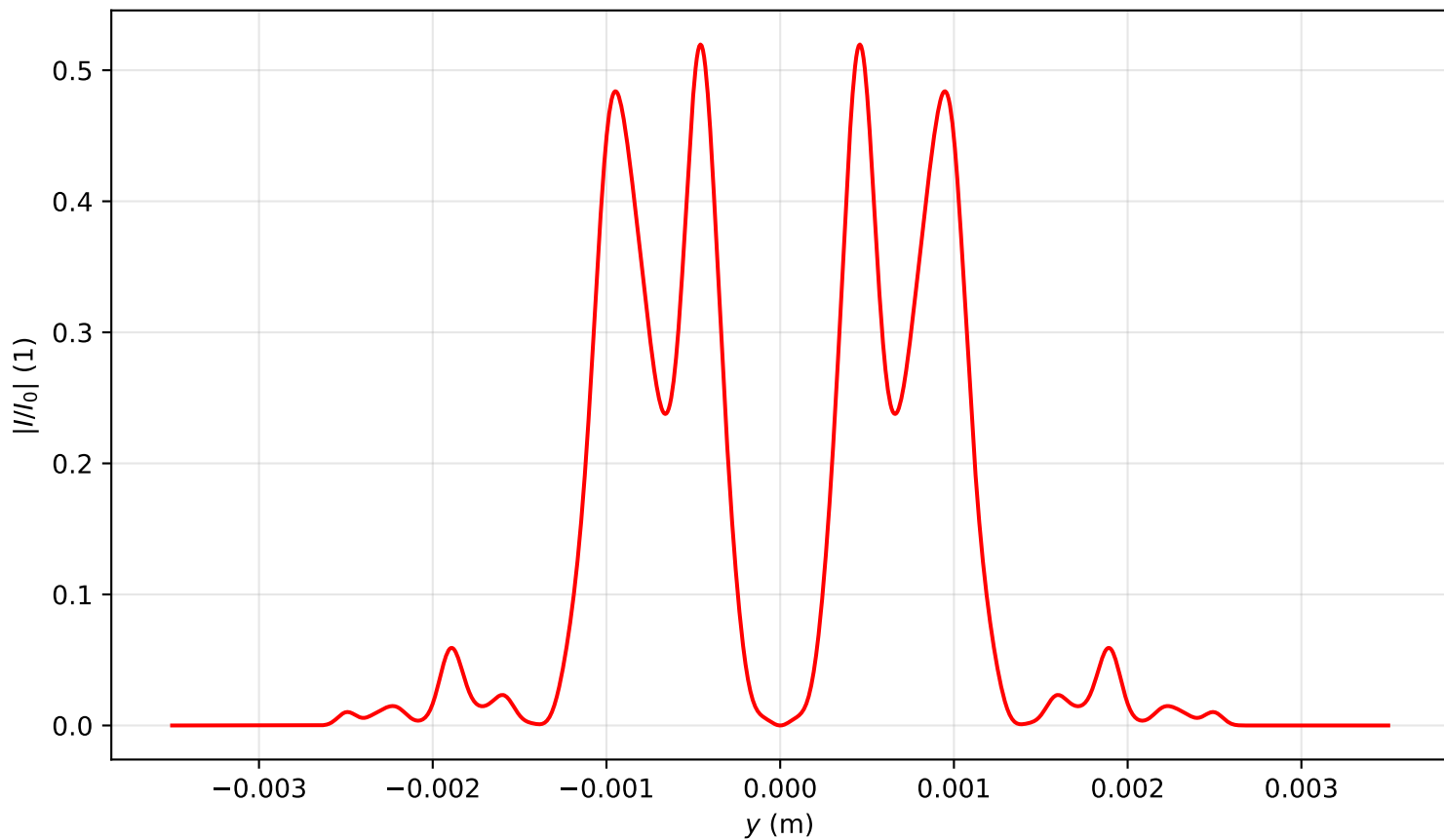
Intensity profile I(x=0, y, z=2.309)/I_0 , P_{in}=15.0P_{cr} , artificial time
