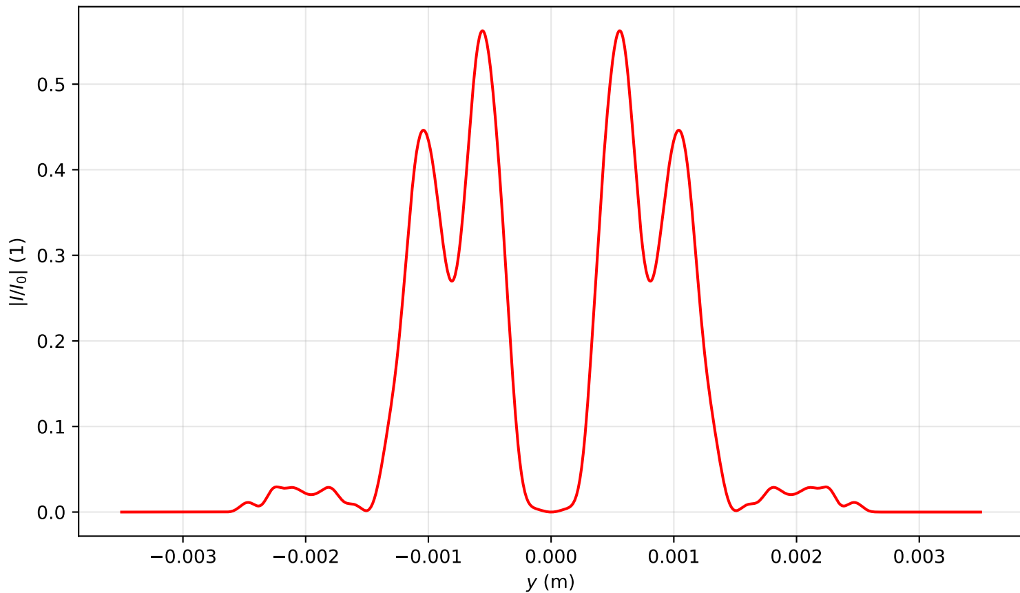
Intensity profile I(x=0, y, z=2.468)/I_0 , P_{in}=15.0P_{cr} , artificial time
