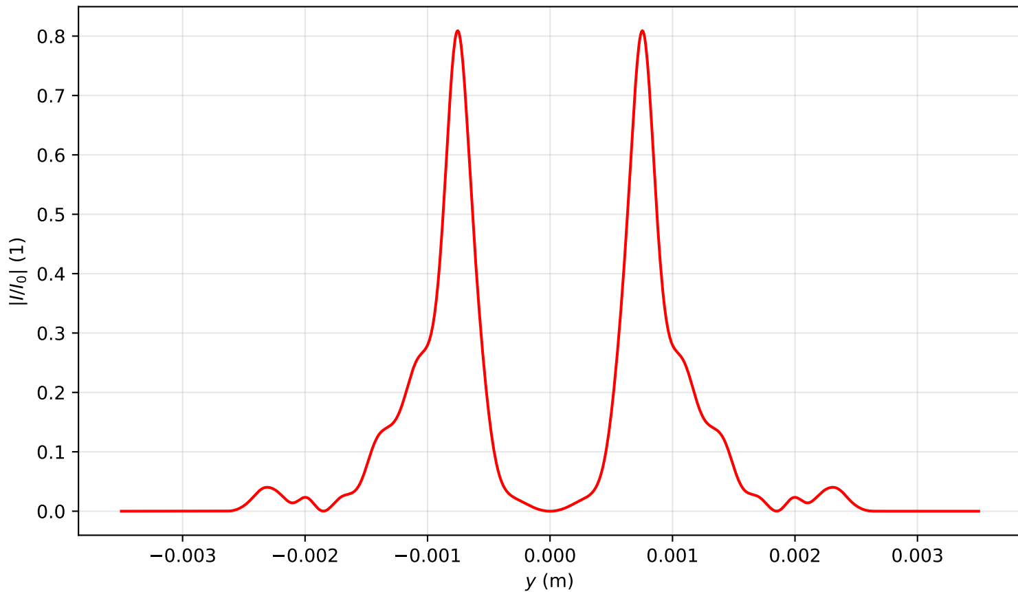
Intensity profile I(x=0, y, z=2.786)/I_0 , P_{in}=15.0P_{cr} , artificial time
