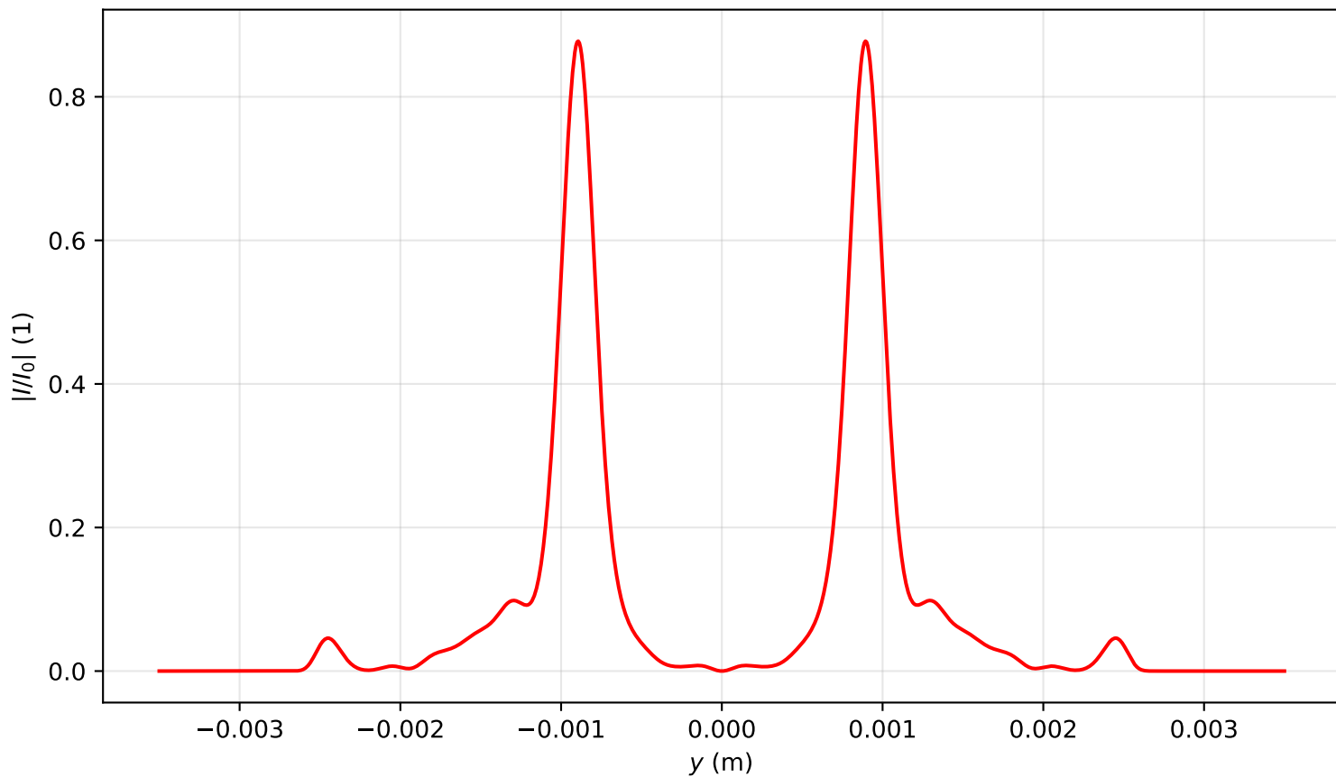
Intensity profile I(x=0, y, z=3.105)/I_0 , P_{in}=15.0P_{cr} , artificial time
